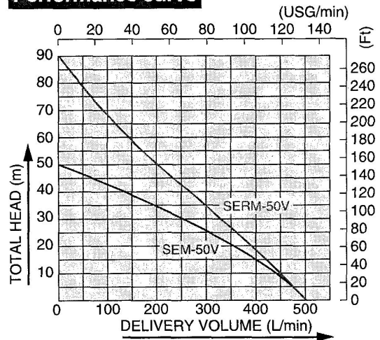
Performance curve
